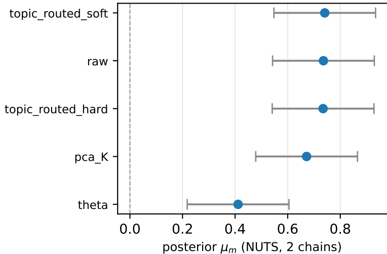
(a) Labelled scenes: 6 scenes x 5 folds x 5 methods
