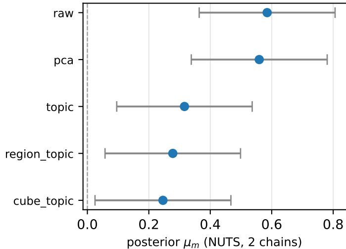
(b) HIDSAG: 5 subsets x 19 targets x 5 methods
