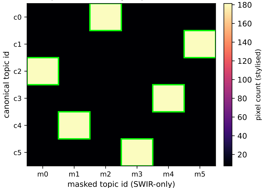
Hungarian alignment on Salinas-A (SWIR mask) paired ARI = 0.766 | swap rate = 0.176
