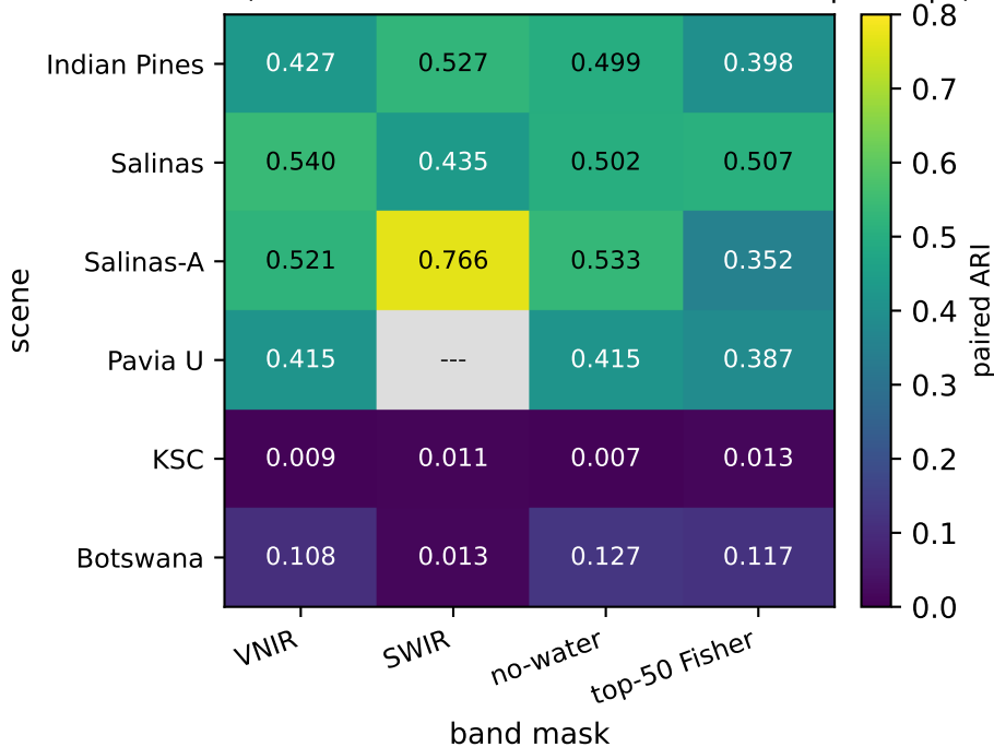
Paired ARI (canonical vs band-masked dominant-topic maps)
