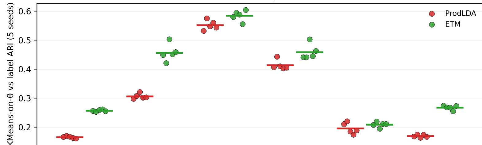
(a) Cluster ARI per seed
