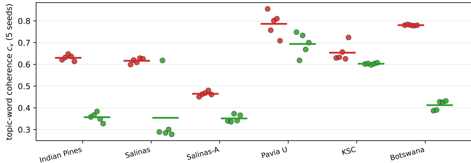
(b) Coherence c_v per seed
