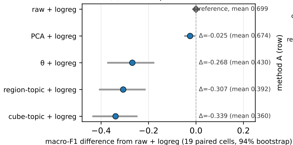
(c) HIDSAG: paired difference
