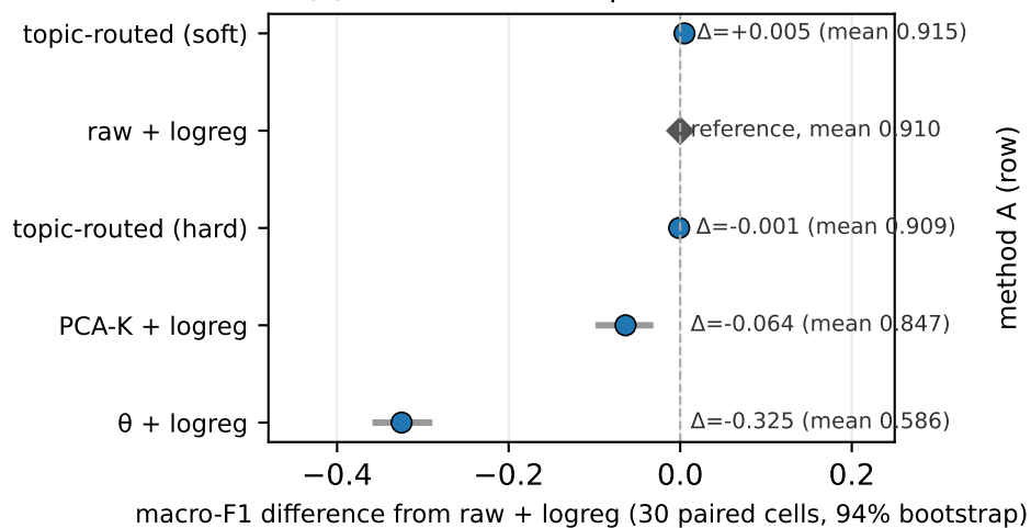
(a) Labelled scenes: paired difference
