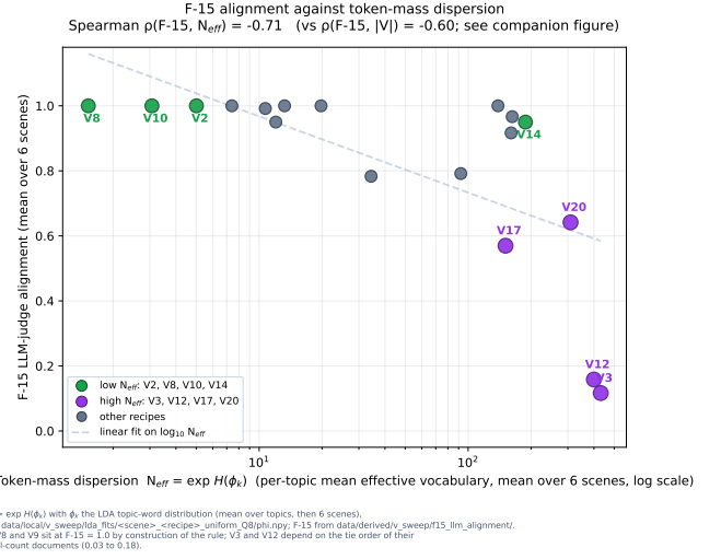
Fig. 1. F-15 LLM-judge alignment versus per-topic mean token-mass dispersion N_{\text{eff}} = \exp(H(\phi_k)) (18), LDA backbone, six labelled scenes, Q = 8 , eighteen recipes (V15 excluded, Table II); the Spearman coefficients in the title are computed over the same eighteen. Point colours are categorical: green for the low- N_{\text{eff}} recipes (V2, V8, V10, V14), purple for the high- N_{\text{eff}} recipes (V3, V12, V17, V20), grey for the others. At the same alphabet size (mean nominal |\mathcal{V}| \approx 1376 ), V3 / V12 / V20 (purple, lower right) fall in dispersion ( 431 > 400 > 309 ) while F-15 is 0.12, 0.16 and 0.64; the V3 and V12 values depend on the order of their tied counts, and V2, V8 and V9 sit at 1.0 by construction (Table III), so the plotted association mixes dispersion with the rule’s construction effects.
