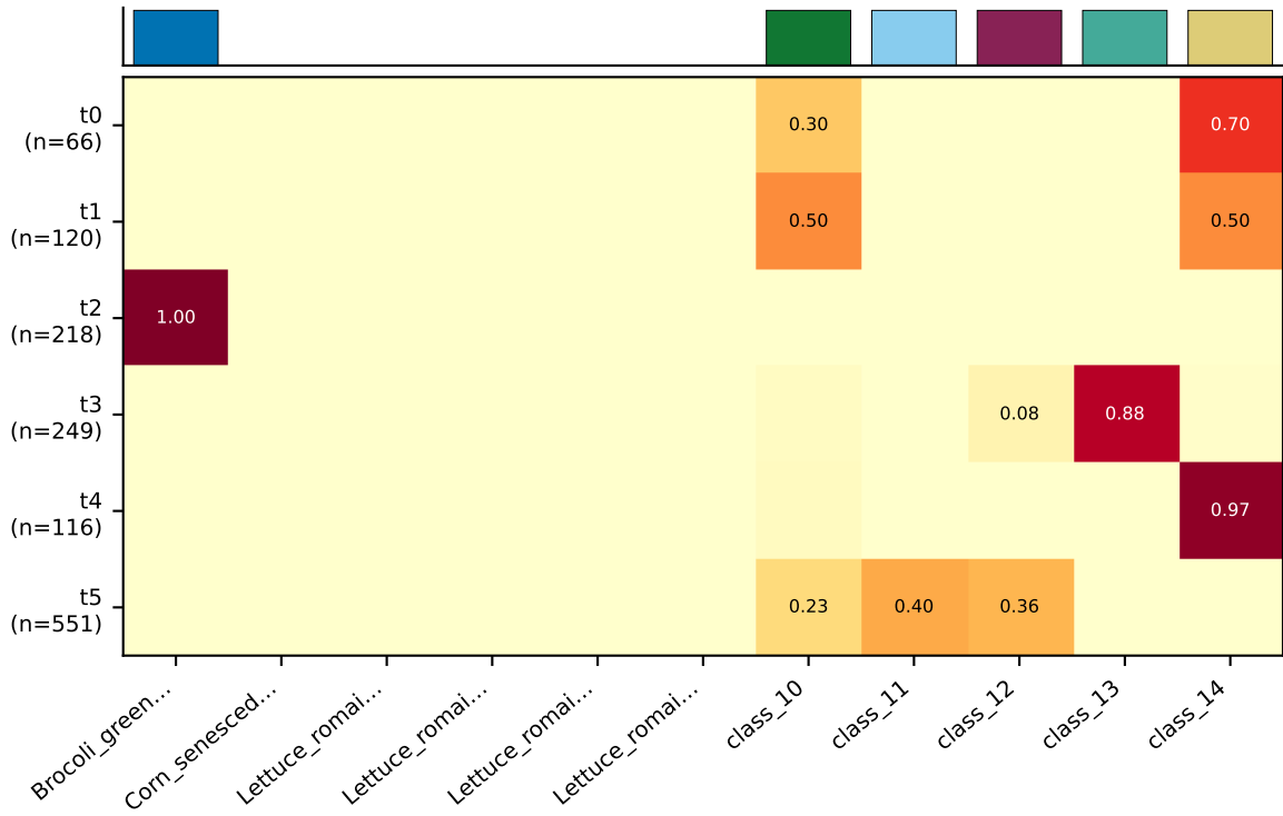
KSC
