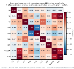
Fig. 6. Spearman rank correlation across the 114 (recipe, scene) cells. F-14 inverted so all axes read “higher = better”. F-2 / ETM and F-2 / ProdLDA cluster tightly ( \rho \geq 0.76 ); F-14 anti-correlates with F-18 ( \rho = -0.74 , the vocabulary-size confounder); F-22 / F-7 correlate at \rho = 0.58 (robust topics tend to be label-aligned).
