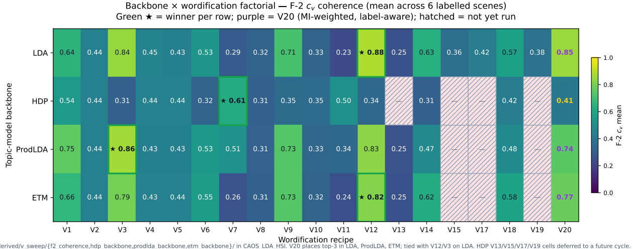
Fig. 6. Backbone \times wordification factorial. Each cell shows the mean F-2 c_v across the six labelled scenes for one (backbone, recipe) pair. Green border + ★ = per-backbone winner; purple cell label = V20 (the label-aware recipe). Hatched cells indicate the (HDP, {V13, V15, V17, V19}) cells that were not re-run in this cycle. No recipe dominates every backbone: LDA + ETM agree on V12 / V3 / V20 ties; HDP picks V7 (sparse absorption tokens); ProdLDA picks V3 with V20 close behind.
