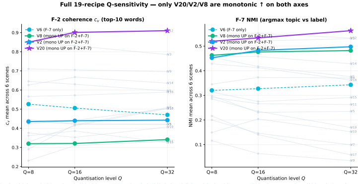
Three recipes climb monotonically on F-2 and F-7 across Q=8/16/32 : V20 (purple *, label-aware), V2 (cyan, intensity-bin), V8 (green, NFINDR endmember). V6 (dashed cyan) climbs on F-7 only — F-2 regresses. V20 has the steepest gains and highest absolute values on both axes. Eight recipes decline monotonically; six peak at Q=16 then regress.
