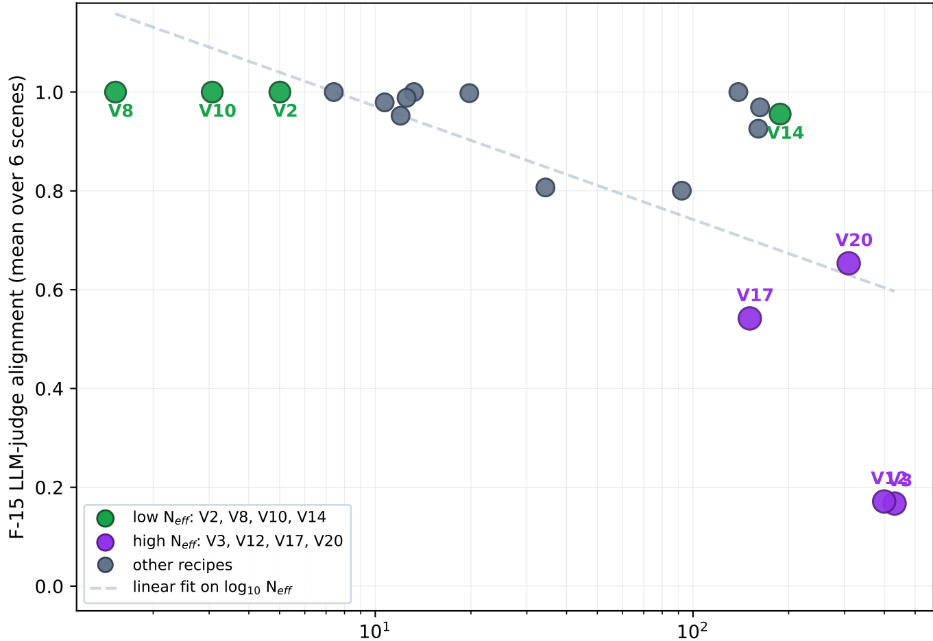
F-15 alignment against token-mass dispersion Spearman \rho(\text{F-15}, N_{\text{eff}}) = -0.77 (vs \rho(\text{F-15}, |V|) = -0.68 ; see companion figure)
