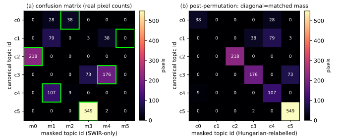
Fig. 3. F-8 Hungarian topic-id alignment on Salinas-A under SWIR-only restriction. Lime rectangles mark the maximum-weight bipartite match \sigma^* ; the diagonal under permutation dominates, consistent with the high paired ARI (0.766) and the low swap rate (0.176) on this (scene, mask) tuple.
