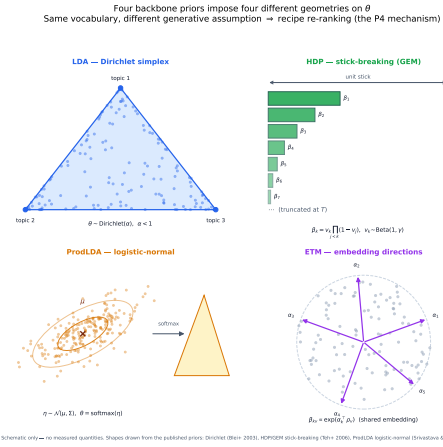
Fig. 3. Why each prior favours a different vocabulary geometry. The Dirichlet-like priors of LDA / ETM (1), (4) reward dense vocabularies (V12 / V3); HDP’s stick-breaking truncation (2) rewards sparse-event vocabularies (V7); ProdLDA’s logistic-normal prior (3) rewards large vocabularies that let a few tokens discriminate strongly (V3).
