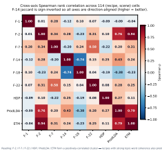
Fig. 7. Spearman rank correlation across the 114 (recipe, scene) cells. F-14 inverted so all axes read “higher = better”. F-2 / ETM and F-2 / ProdLDA cluster tightly ( \rho \geq 0.76 ); F-14 anti-correlates with F-18 ( \rho = -0.74 , the vocabulary-size confounder); F-22 / F-7 correlate at \rho = 0.58 (robust topics tend to be label-aligned).
