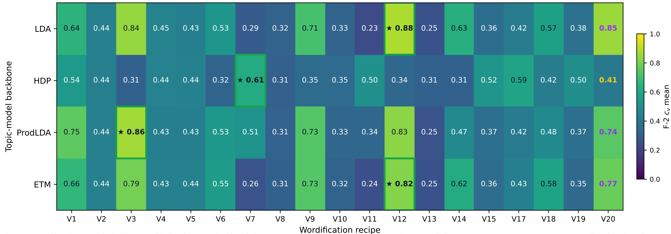
Backbone × wordification factorial — F-2 c_v coherence (mean across 6 labelled scenes) Green ★ = winner per row; purple = V20 (MI-weighted, label-aware); hatched = not yet run
