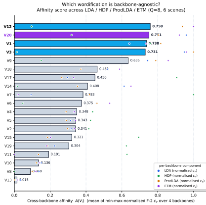
Fig. 2. Cross-backbone affinity \mathcal{A}(V_i) (19) per recipe (Table III). V12 tops the ranking (0.76), V20 second (0.75); V13 has the lowest affinity (0.01), at or near the per-backbone minimum. V20 is the only label-aware recipe in the leading group.
