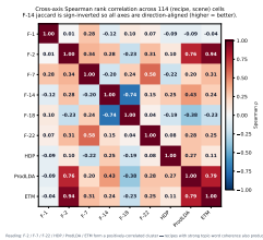
Fig. 6. Spearman rank correlation across the 114 (recipe, scene) cells. F-14 inverted so all axes read “higher = better”. F-2 / ETM and F-2 / ProdLDA cluster tightly ( \rho \geq 0.76 ); F-14 anti-correlates with F-18 ( \rho = -0.74 , the vocabulary-size confounder); F-22 / F-7 correlate at \rho = 0.58 (robust topics tend to be label-aligned).
