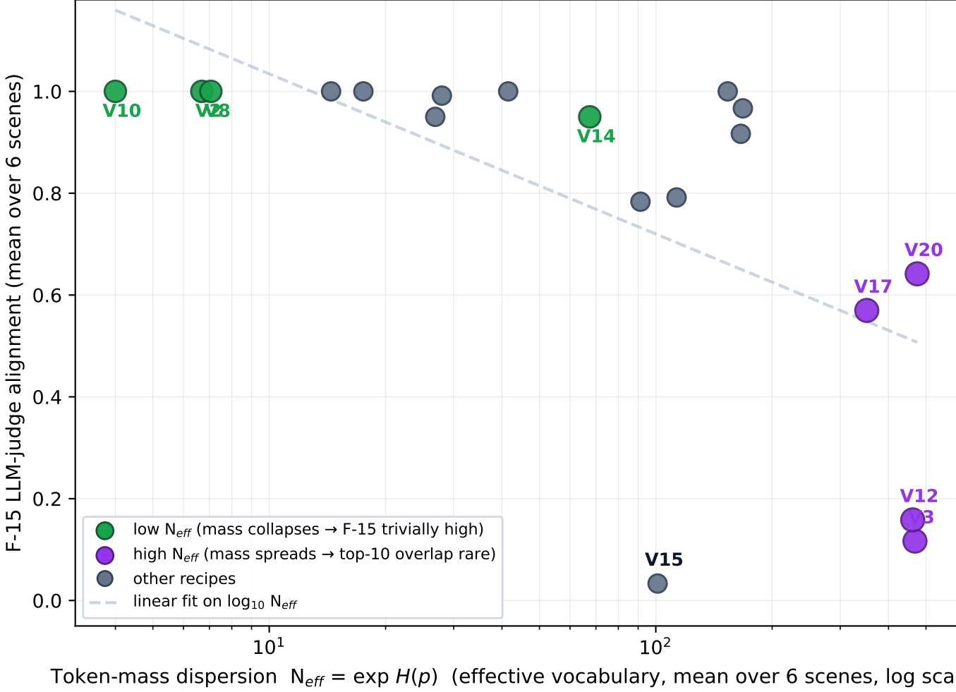
P5 mechanism — F-15 alignment tracks token-mass dispersion, not coherence Spearman \rho(\text{F-15}, N_{\text{eff}}) = -0.73 (vs \rho(\text{F-15}, |V|) = -0.57 ; see companion figure)
