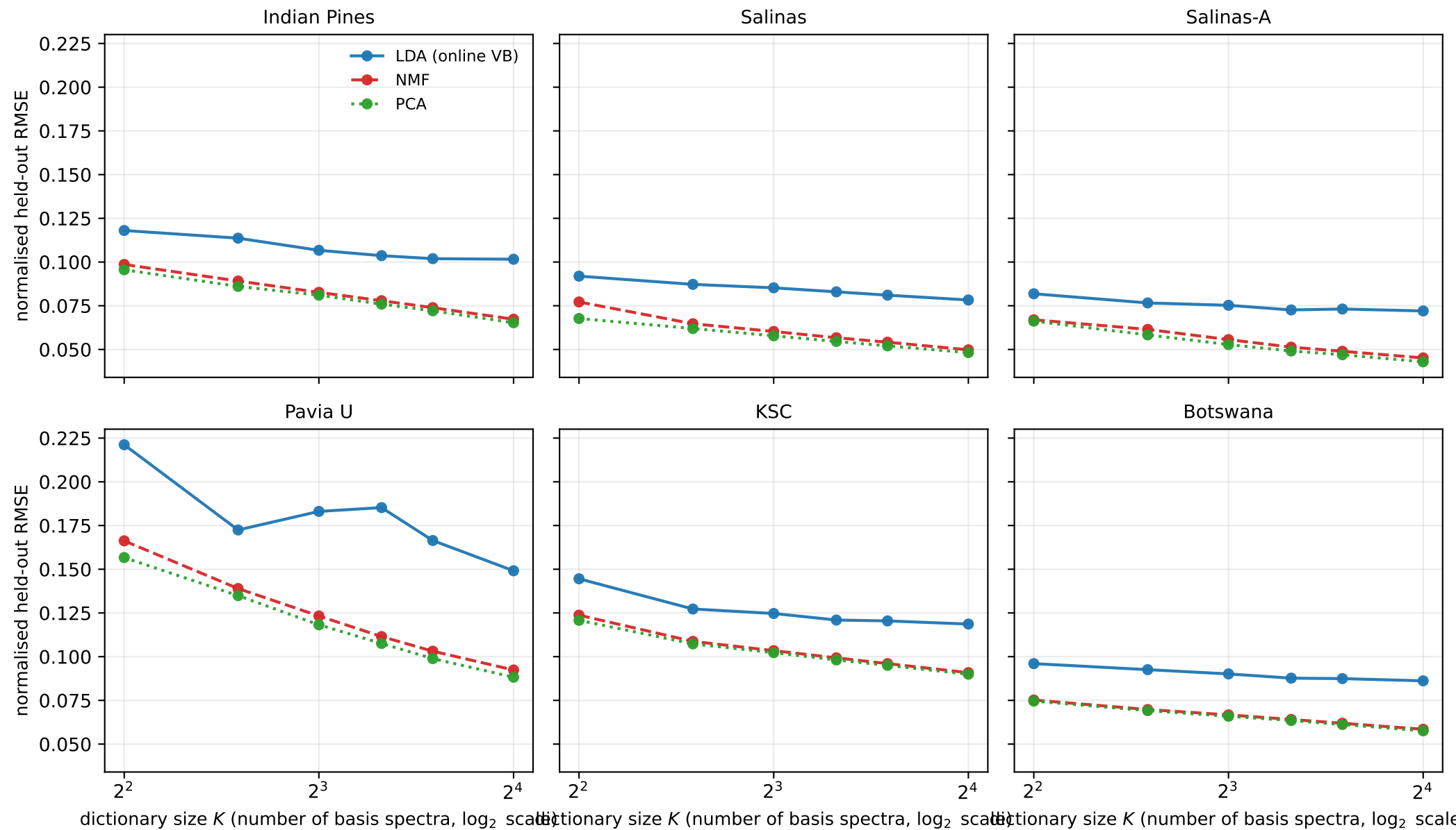
F-11 distortion vs dictionary size K of \theta — LDA vs NMF vs PCA per scene
