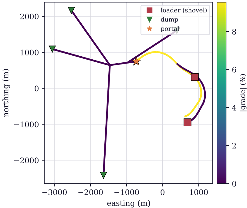
generated open-pit haul network
