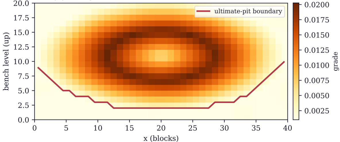
porphyry twin: grade field + exact ultimate pit (22026 of 32000 blocks)
