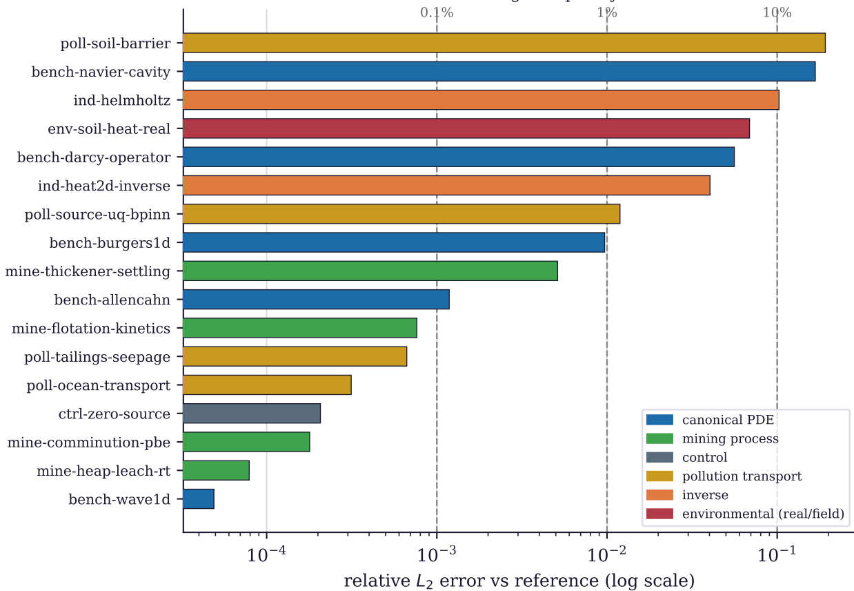
PINN accuracy atlas: sub-percent on smooth forward PDEs, orders worse on inverse / high-frequency / real-data cases
