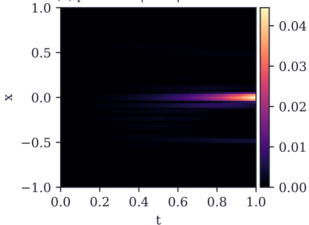
(b) pointwise |\text{error}| vs reference
