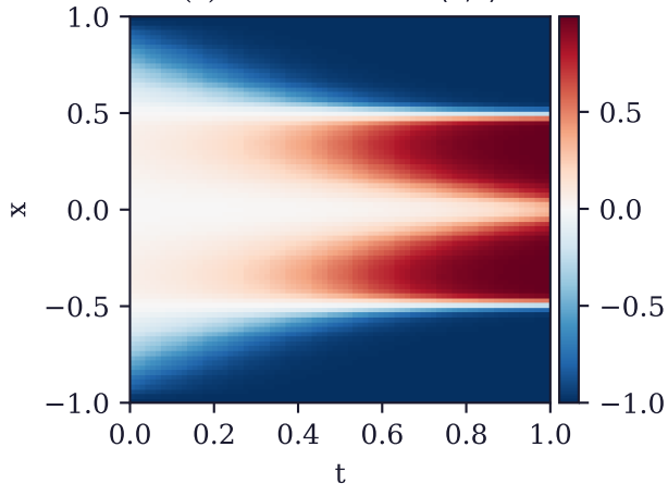
(a) PINN solution u(x, t)
