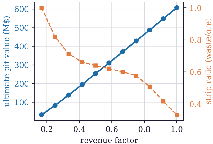
(a) Whittle nested pit shells (Porphyry copper (disseminated shell))
