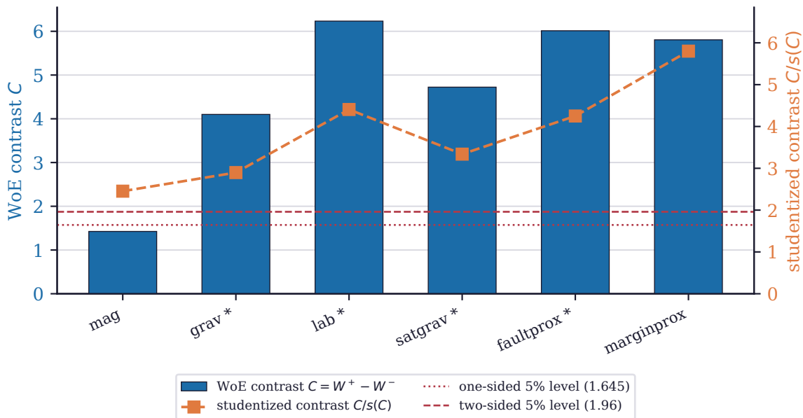
Real US-MVT: WoE contrasts and studentized contrasts
