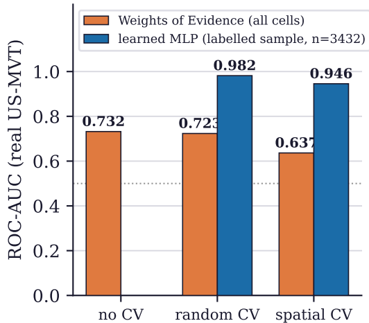
(b) real belt: AUC by protocol
