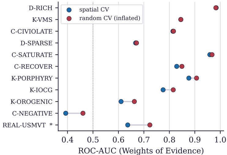
(a) random CV inflates the AUC; spatial CV is the realistic estimate
