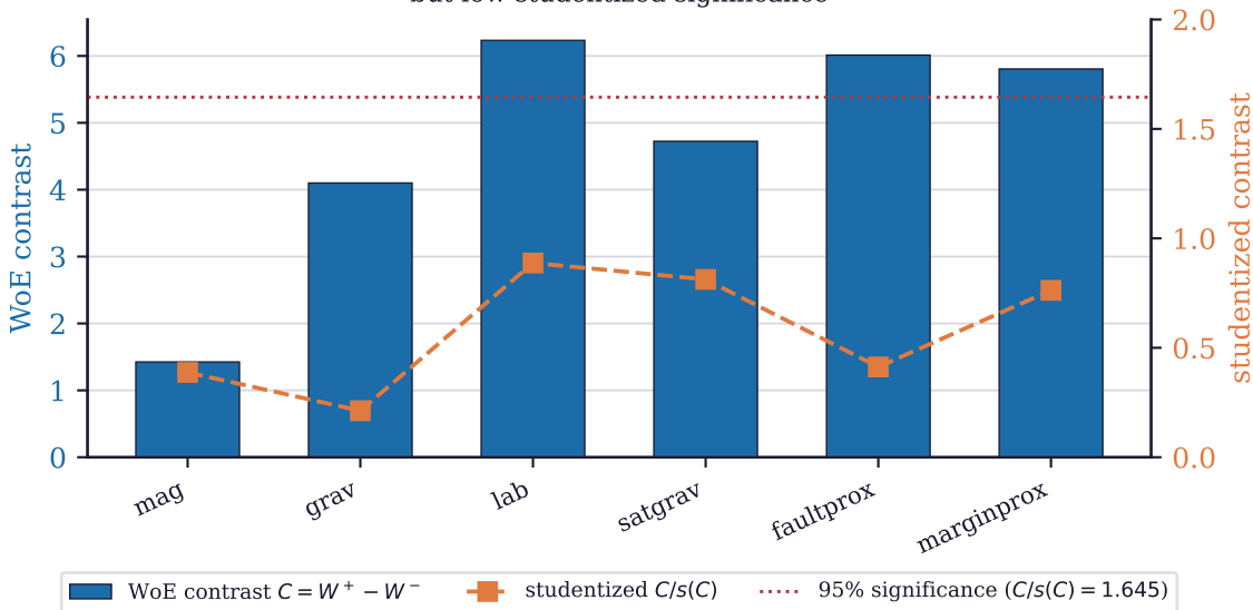
Real US-MVT: large WoE contrasts, but low studentized significance
