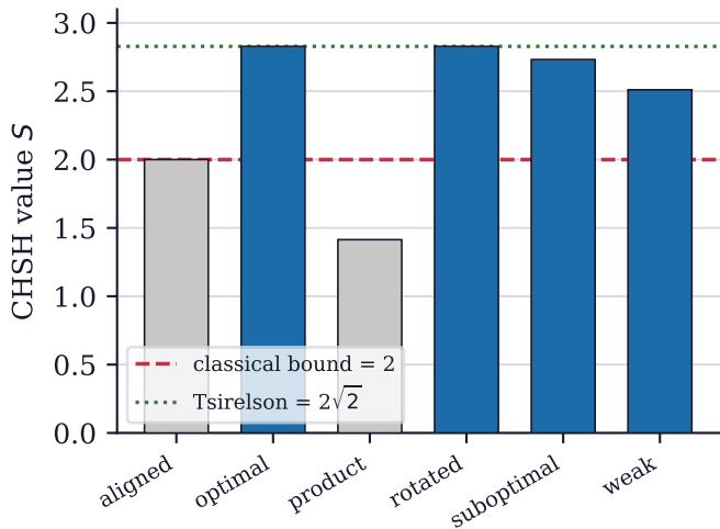
(a) CHSH: quantum genuinely violates the classical bound
