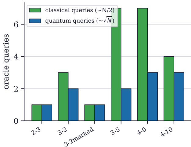
(b) Grover: fewer queries (asymptotic, not wall-time)
