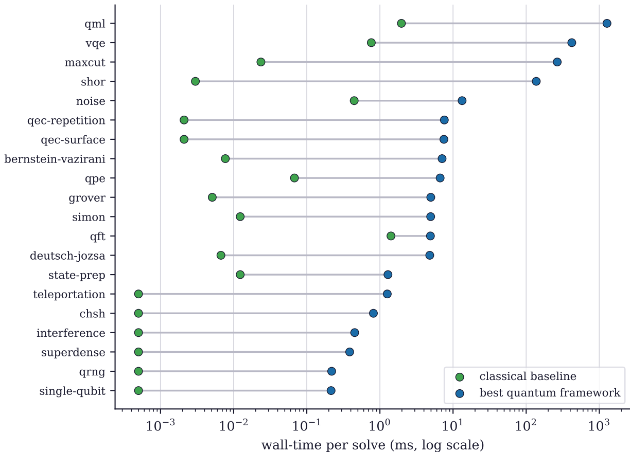
classical wins wall-time on all 20 problems (lab scale)
