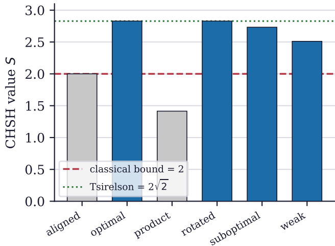
(a) CHSH: quantum violates the classical bound
