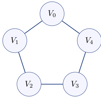
Figure 1: The five-type obstruction. Lines show allowed adjacencies, not an assumption of complete bipartite adjacency.
