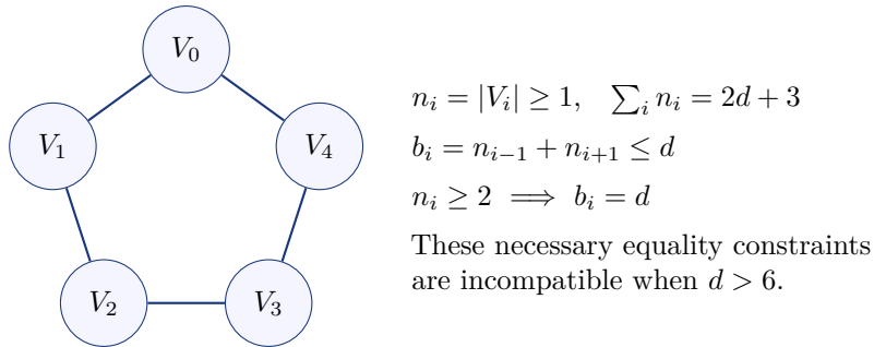
Figure 1: The five-type obstruction. Lines show allowed adjacencies, not an assumption of complete bipartite adjacency.
