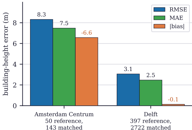
Fused heights against 3D BAG LoD2
