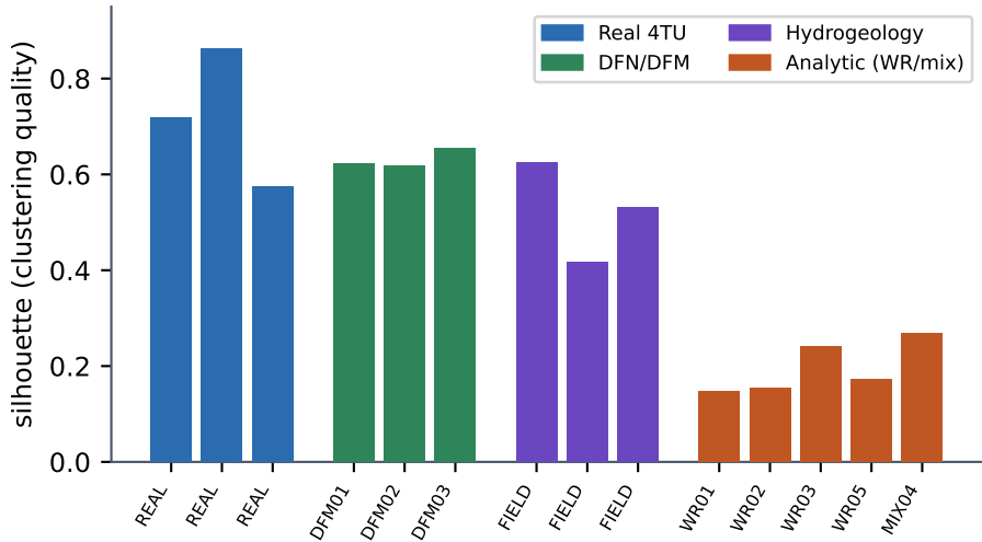
Real transients cluster more cleanly than analytic families
