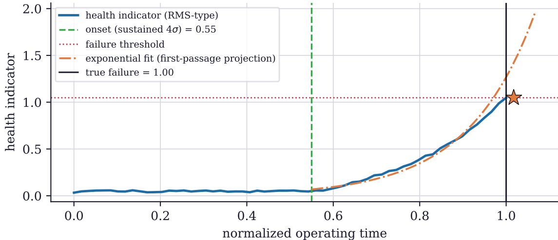
first-passage RUL on a controlled degradation (method illustration)
