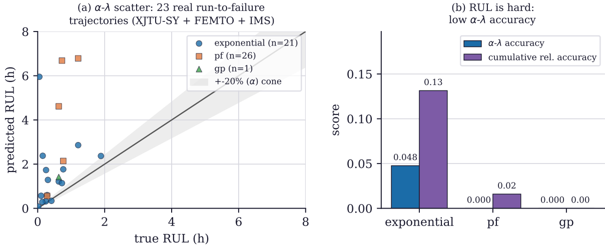
Fig. 3. RUL on 23 real run-to-failure trajectories (XJTU-SY, FEMTO, IMS) under the Saxena \alpha - \lambda protocol. (a) Predicted versus true RUL at the life-fraction checkpoints, with the \pm 20\% ( \alpha ) accuracy cone: most predictions fall outside it, and the particle filter in particular scatters far (predicting several hours of life when under one remains). (b) The resulting \alpha - \lambda accuracy and cumulative relative accuracy per model: the best (exponential first-passage) is 0.048 and 0.13; the probabilistic models are worse. The low scores reflect the task, not a tuning failure.
