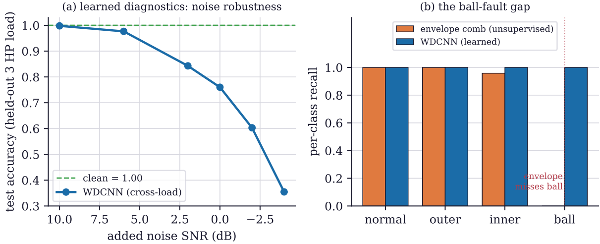
Fig. 1. Bearing diagnostics on the CWRU data. (a) The learned WDCNN, trained on three motor loads and tested on the entire held-out fourth, is perfect on clean signals and degrades gracefully as noise is added, from 1.00 accuracy to 0.35 at -4 dB signal-to-noise ratio. (b) Per-class recall of the leakage-immune unsupervised envelope comb versus the learned WDCNN: the envelope method reaches recall 1.00, 1.00 and 0.96 on healthy, outer-race and inner-race classes but fails entirely on ball faults (recall 0.00), the hard case where the ball-fault modulation is smeared across the spectrum; the learned model recovers it.
