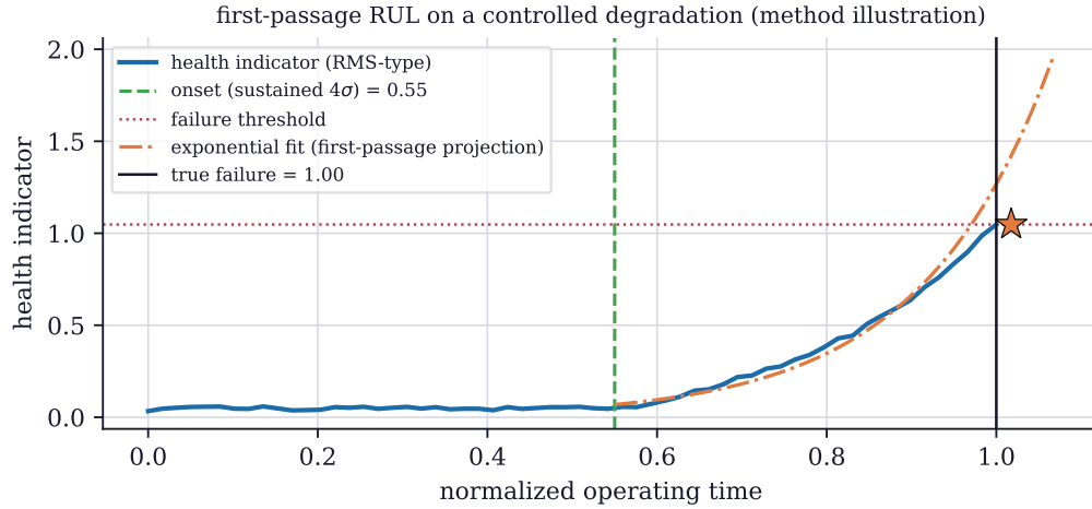
Fig. 2. The first-passage RUL method on a controlled degradation (method illustration). A scalar health indicator is trended; onset is declared at the first sustained 4\sigma excursion above the healthy baseline (two consecutive points, so a single spike does not trigger it); an exponential is fit to the post-onset points in log space and accepted only if its slope is positive; and the RUL is the time from now to when the fit first crosses the failure threshold. On a clean degradation the projection (star) lands on the true failure. Real bearings are not this clean.
