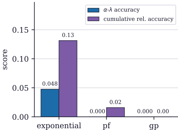
(b) RUL is hard: low \alpha - \lambda accuracy (the honest record)
