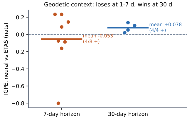
Fig. 3. The strain-conditioned neural challenger vs ETAS in the pseudo-prospective back-analysis. Per-window IGPE is scattered around zero at seven days (mean -0.053 , only 4/8 positive) but positive in every window at thirty days (mean +0.078 ). Read from neural_pseudoprospective.json .
