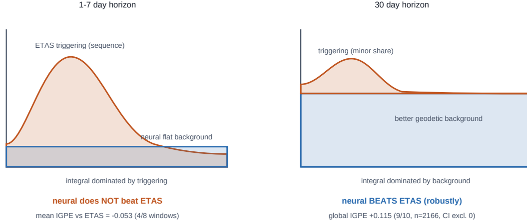
Fig. 5. Mechanism of the horizon dependence. The calibrated neural’s total forecast is constant across windows (18.1 events at seven days, 77.3 at thirty, ratio \approx 30/7 ): it deploys a time-flat geodetic background , not a triggering model. At the short horizon the integral is dominated by ETAS triggering, which the flat background cannot track (neural loses); at the long horizon the integral is dominated by the background, where a better geodetic background wins.
