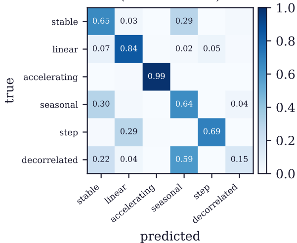
(b) deformation-type confusion (macro-F1 0.556)
