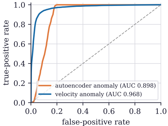
(a) anomaly detection
