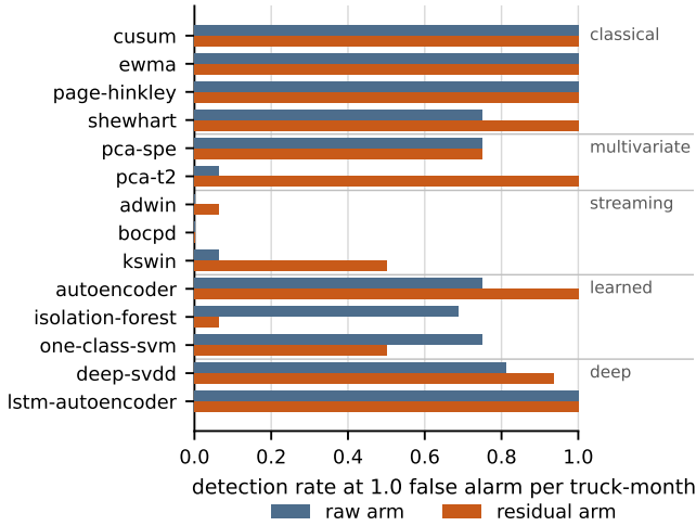
Fig. 2. The fourteen-rung ladder at a matched budget, by tier. Conditioning helps six rungs (largest: Hotelling T^2 , 0.06 \rightarrow 1.00 ), leaves the detection rate of six unchanged (four at ceiling, SPE at 0.75, BOCPD at zero) and hurts two learned novelty models. BOCPD detects nothing on either arm (gradual ramps against an abrupt-change model); ADWIN’s integer statistic leaves it only d+1 operating points.
