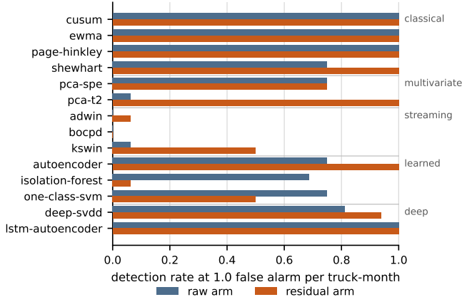
Fig. 2. The complete fourteen-rung ladder at a matched budget, by tier. Conditioning helps six rungs (largest: Hotelling T^2 , 0.06 \rightarrow 1.00 ), leaves six at ceiling, and hurts two learned novelty models. BOCPD detects nothing on either arm (gradual ramps against an abrupt-change model); ADWIN’s integer statistic leaves it only d+1 operating points.
