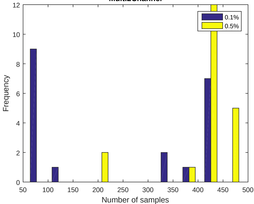
Multi2Channel
