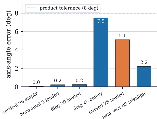
(a) orientation recovered across paths (mean 2.5 deg; orange = curved)
