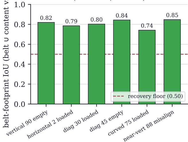
(b) belt region recovered (mean 0.81, min 0.74)
