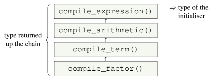
Figure 4: Each precedence level returns the type tag of the value it compiled. The type auto needs is the return value of compile_expression() .
