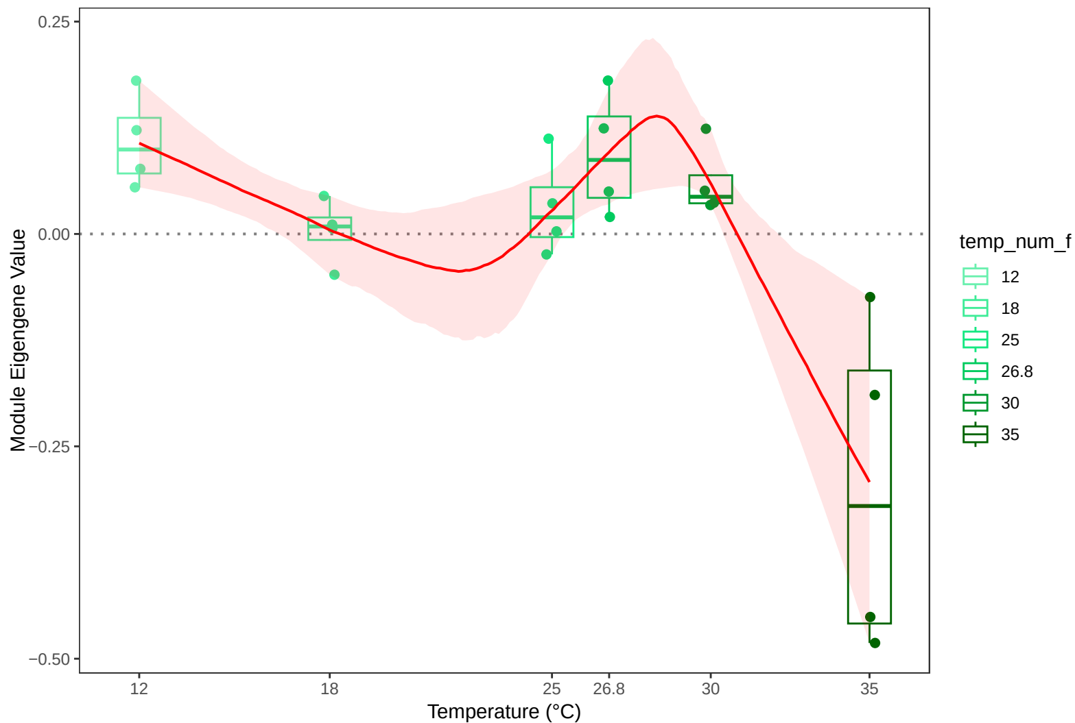
Module5: Strader Plot with Bootstrapped Segmented Regression CI
