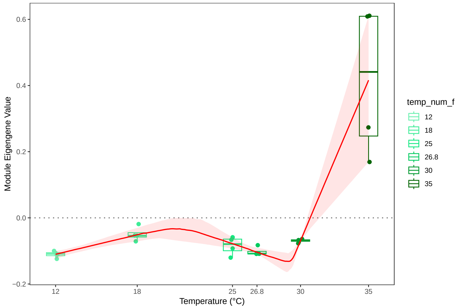
Module8: Strader Plot with Bootstrapped Segmented Regression CI
