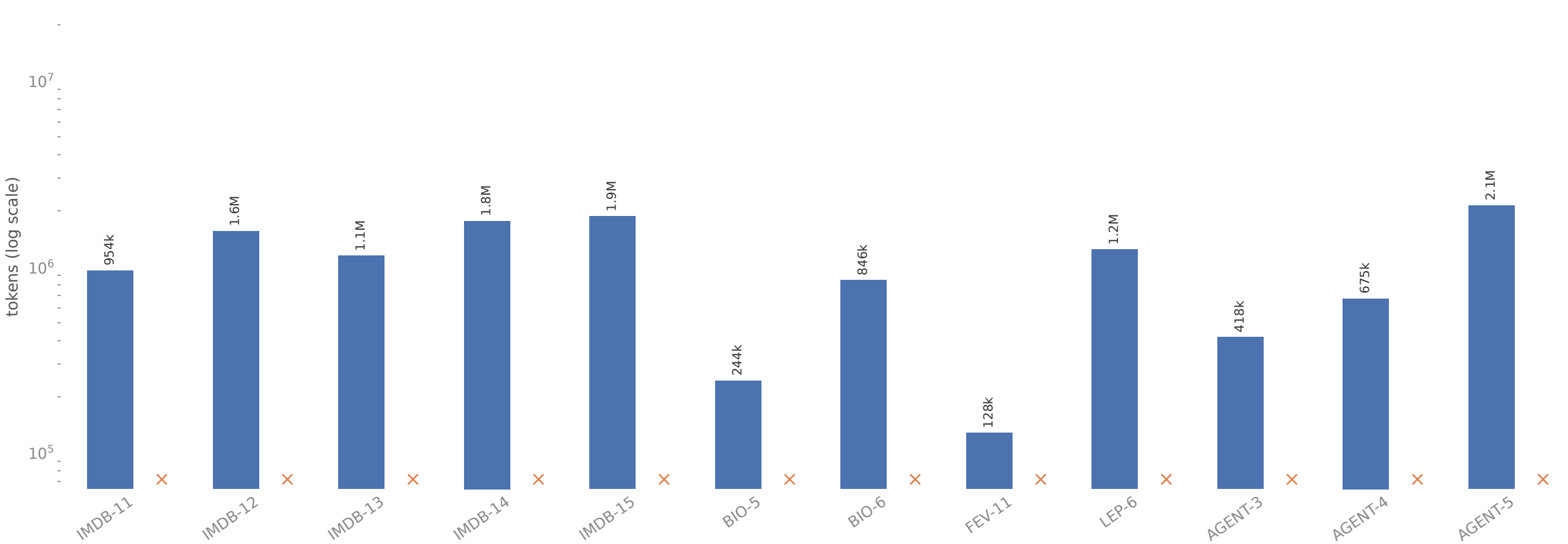
KV regret: fresh tokens minus the token minimum (SoL is 0 by definition)
