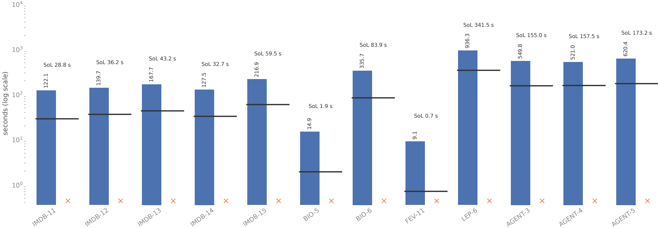
Latency: query time with planning, without model startup
