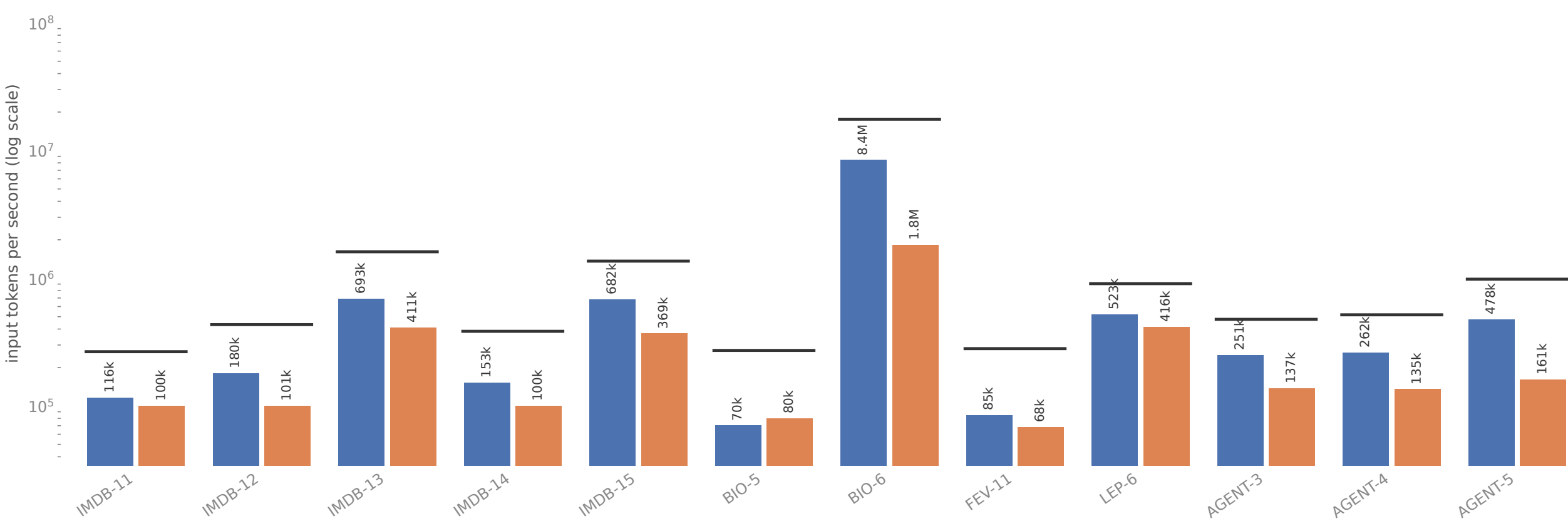
Throughput: every prompt's full input length over query time
