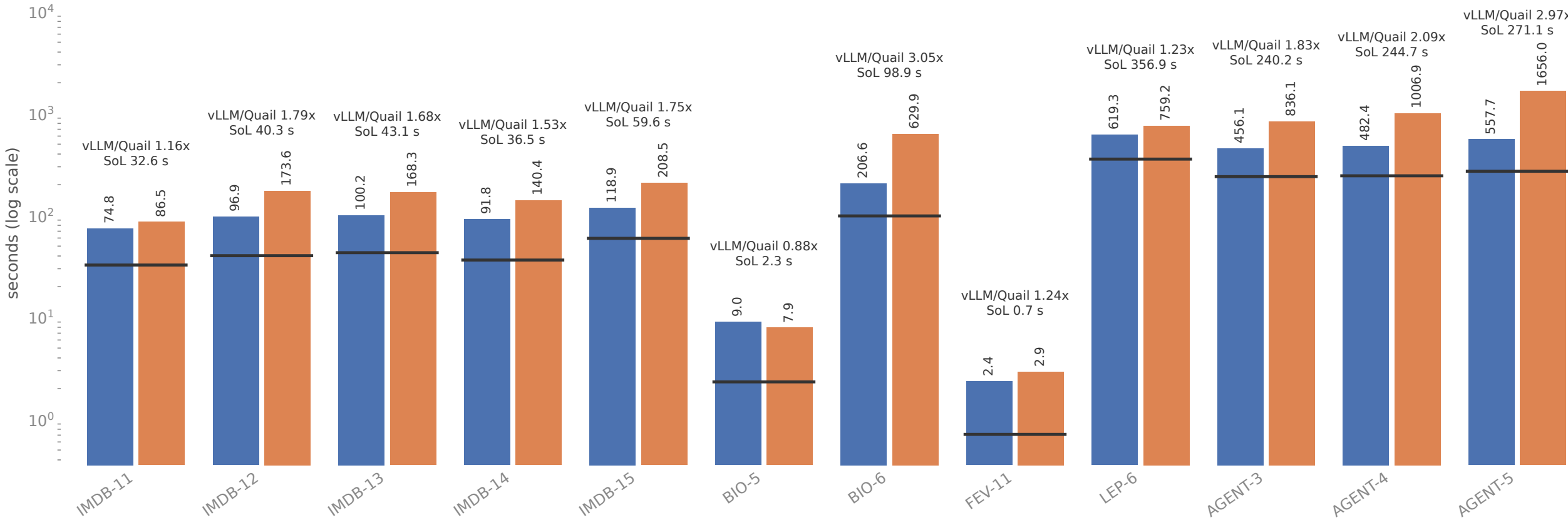
Latency: query time with planning, without model startup
