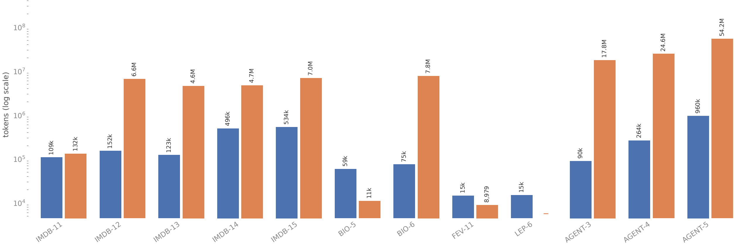
KV regret: fresh tokens minus the token minimum (SoL is 0 by definition) ; stock vLLM's is approximate
