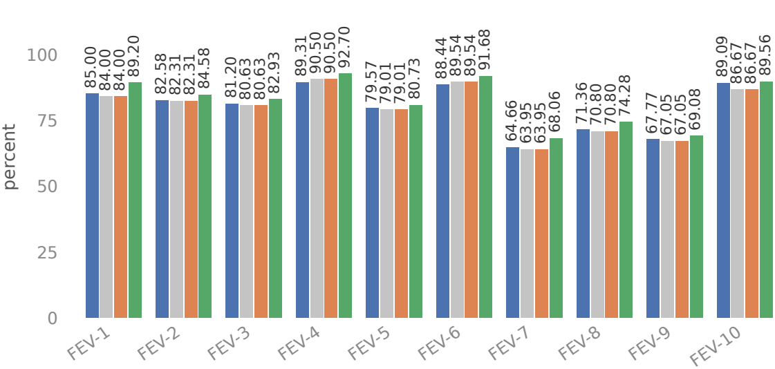
Answer agreement with Qwen3 32B
