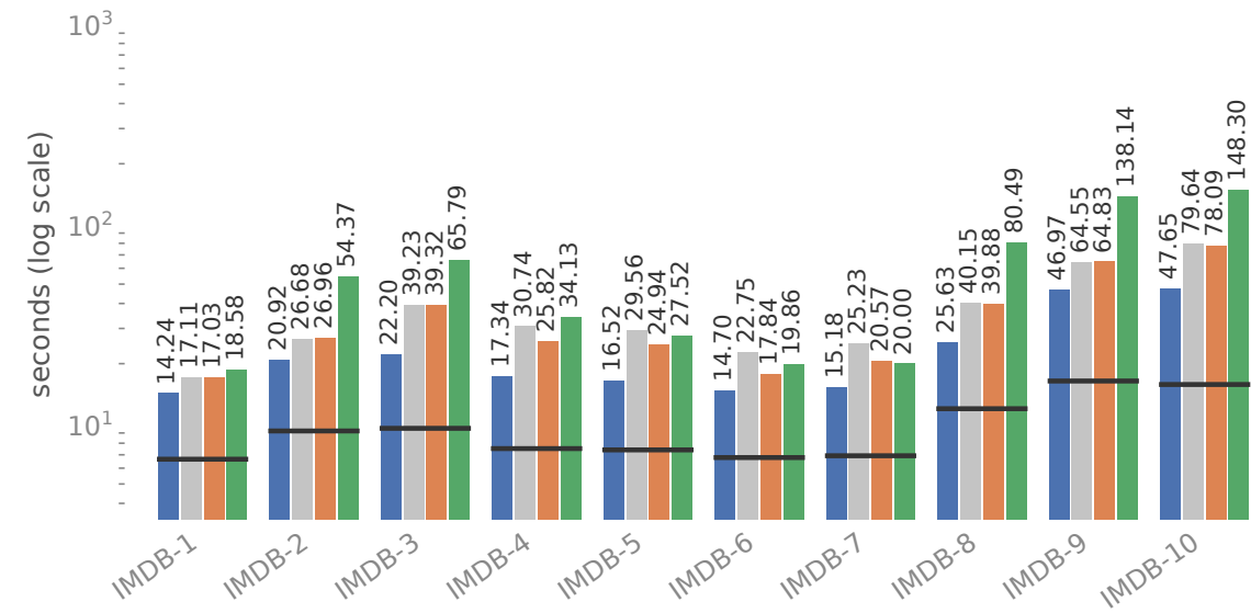
Latency
