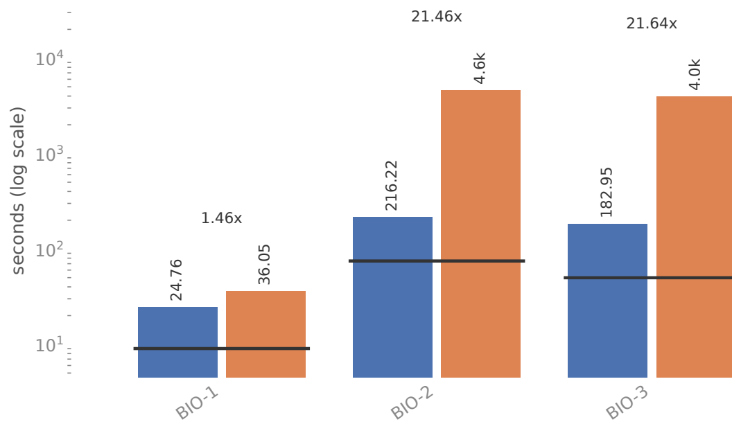
Latency (ratios: vLLM / Quail)
